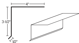
Eave Trim
