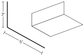
High Side Transition
