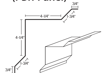
Inside Corner Trim (PBR-Panel)
