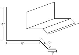
Rake Transition
