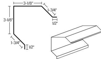
Outside Corner Trim (PBR-Panel)
