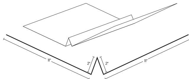
Standard Valley
