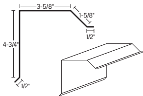
Rake Trim
