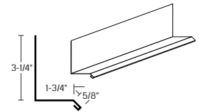
Base Trim
